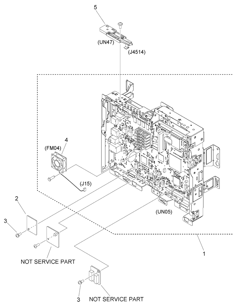
Figure 930C MAIN CONTROLLER PCB ASSEMBLY (C3720)
