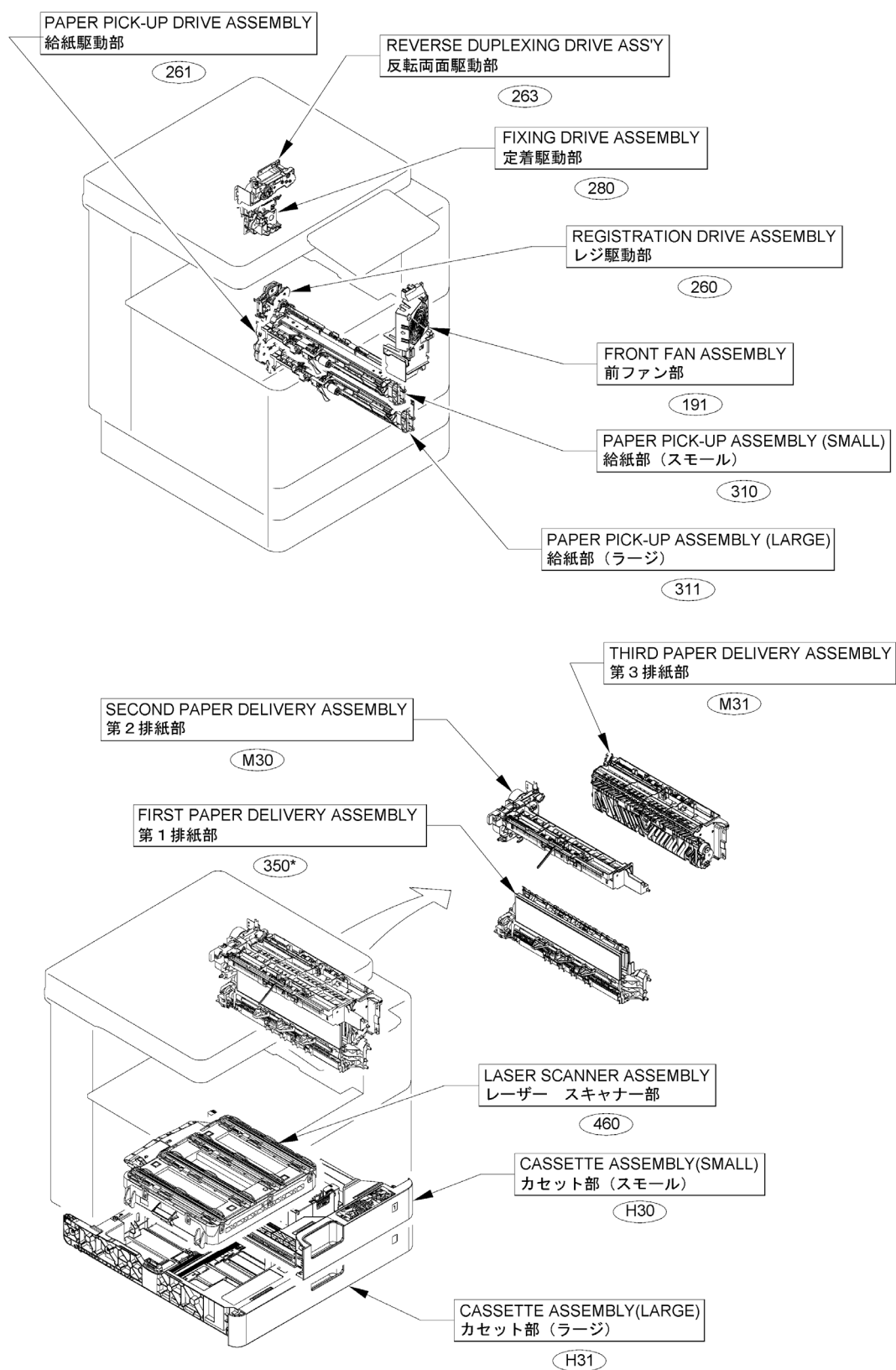
Figure A1C (2/4) ASSEMBLY LOCATION DIAGRAM
