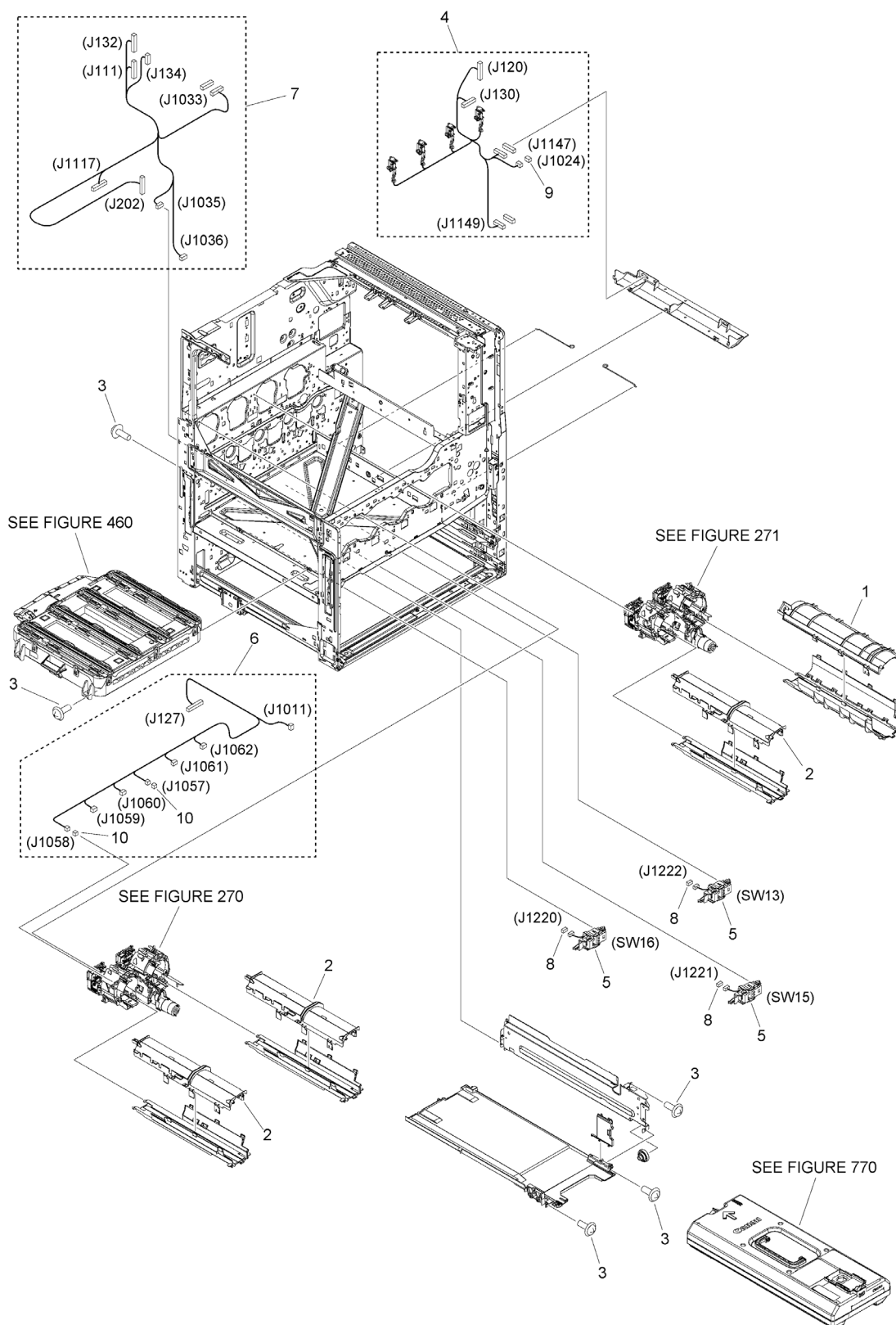
Figure 103 INTERNAL COMPONENTS 3
