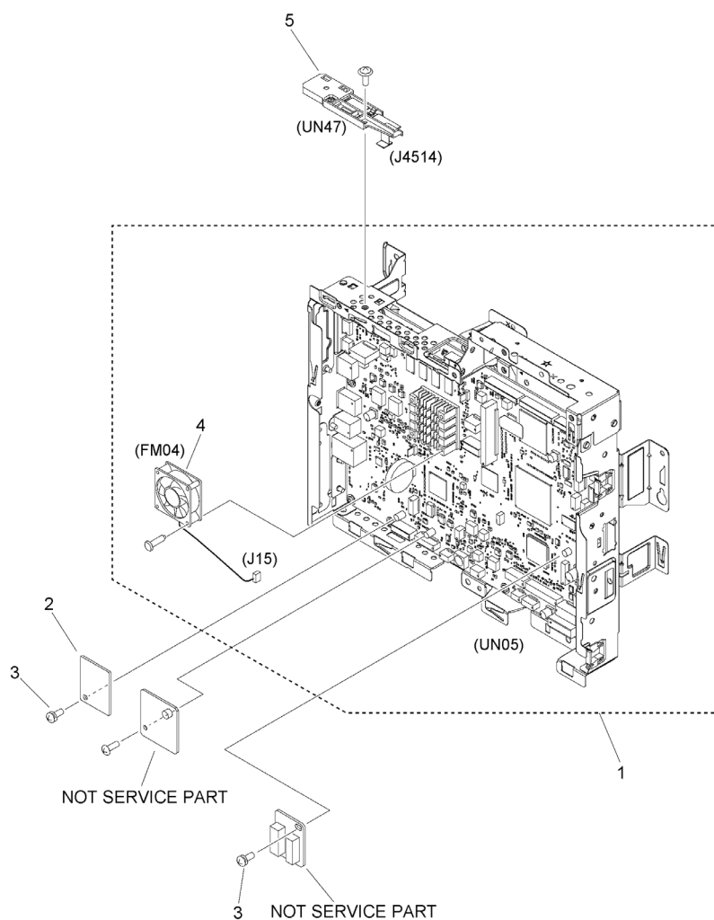
Figure 930A MAIN CONTROLLER PCB ASSEMBLY (C3730)
