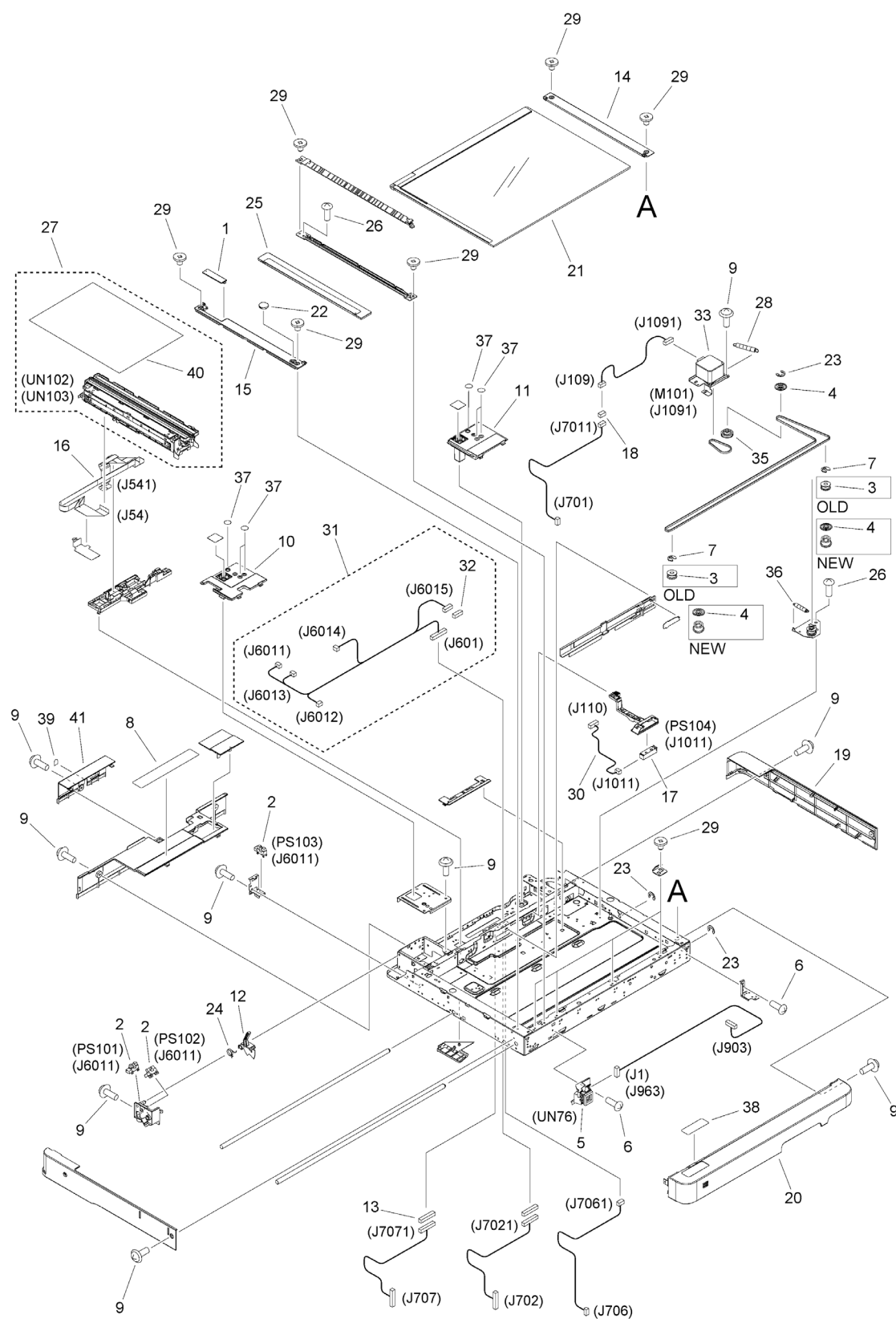
Figure D11J READER ASSEMBLY
