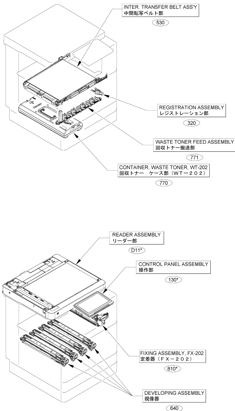
Figure A1C (3/4) ASSEMBLY LOCATION DIAGRAM
